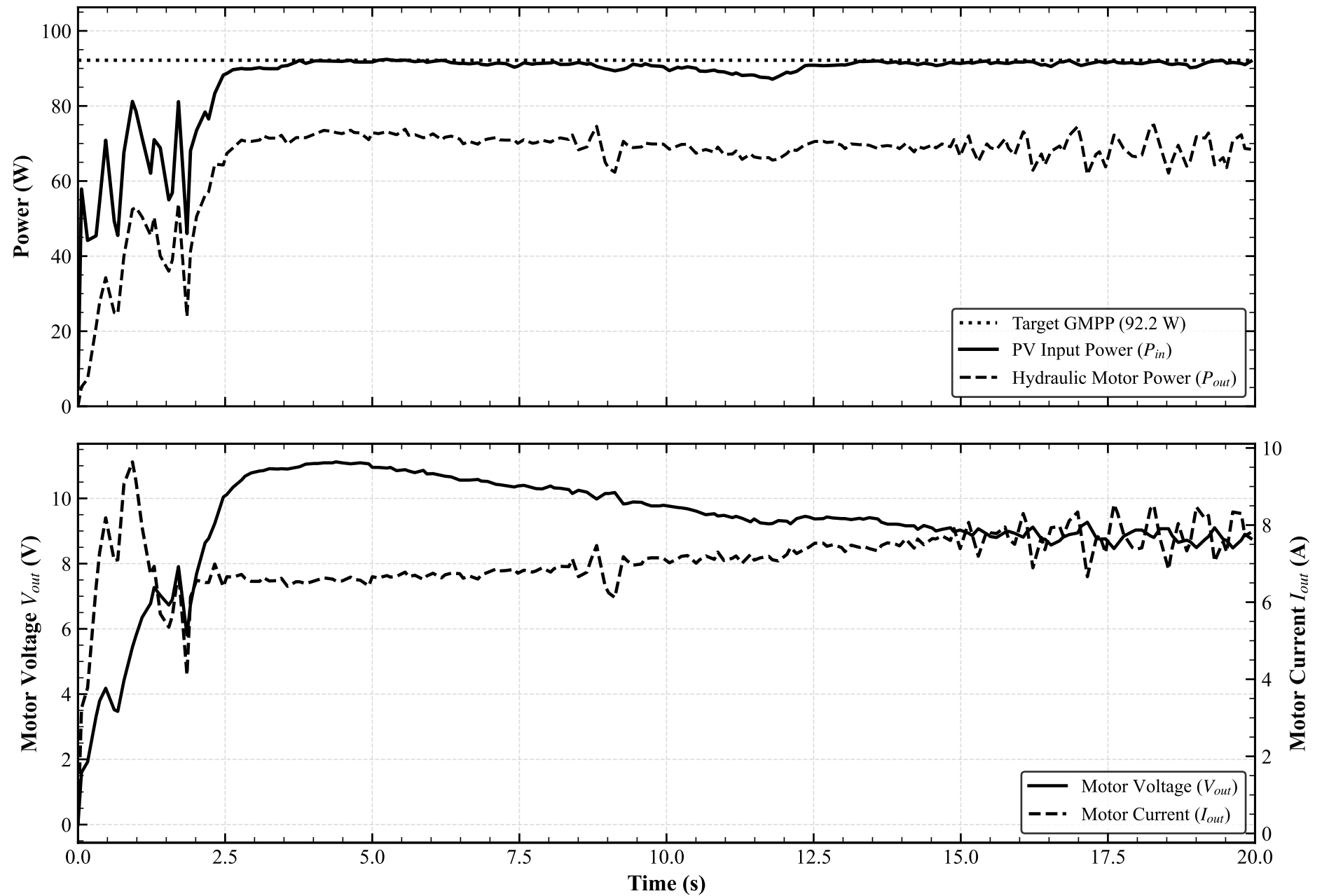
Hydraulic System Response — Level 2 (Shading - 660 W/m 2 )
